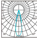
Luminous flux luminaire 1224lm (EXTREME CUT OFF)
