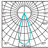
Luminous flux luminaire 1209lm (EXTREME CUT OFF)
