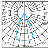
Luminous flux luminaire 1149lm (EXTREME CUT OFF)
