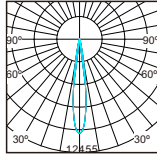
Luminous flux luminaire 1100lm (EXTREME CUT OFF)
