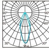
Luminous flux luminaire 223lm (EXTREME CUT OFF)
