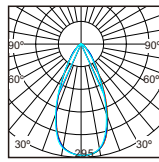
Luminous flux luminaire 235lm (EXTREME CUT OFF)
